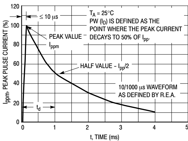
Figure 11. Pulse Waveform
