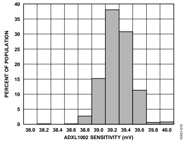
Figure 15. ADXL1002 Sensitivity Histogram at 25°C
