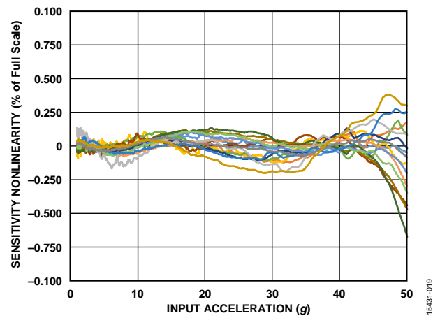
Figure 20. ADXL1002 Sensitivity Nonlinearity vs. Input Acceleration
