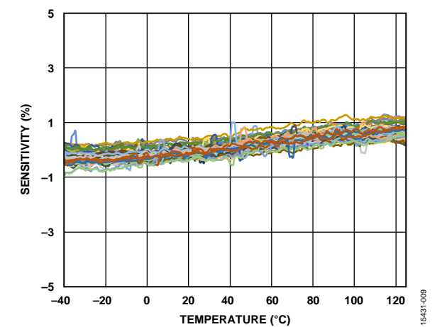
Figure 9. ADXL1002 Sensitivity vs. Temperature
