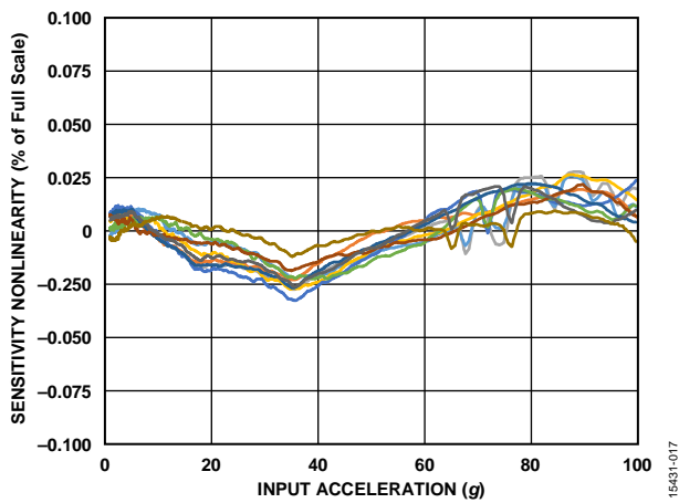
Figure 17. ADXL1001 Sensitivity Nonlinearity vs. Input Acceleration
