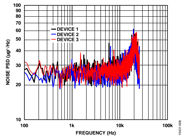
Figure 8. ADXL1002 Noise Power Spectral Density (PSD)
