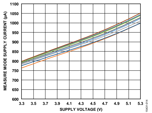
Figure 14. ADXL1001/ADXL1002 Measure Mode Supply Current vs. Supply Voltage
