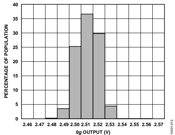
Figure 21. ADXL1001/ADXL1002 0g Output Population
