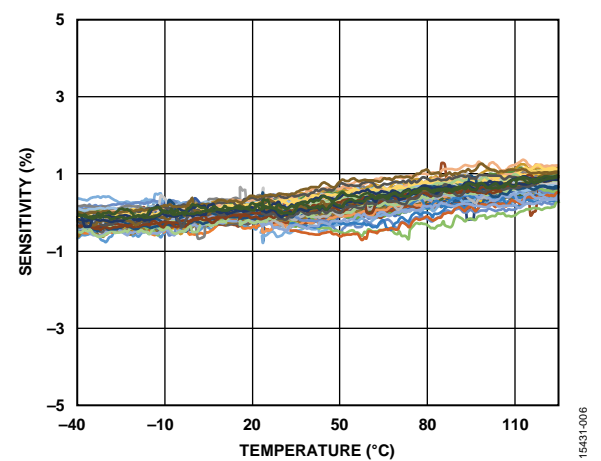
Figure 6. ADXL1001 Sensitivity vs. Temperature
