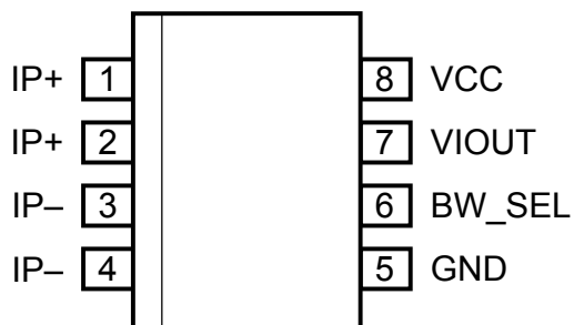
Pinout Diagram
