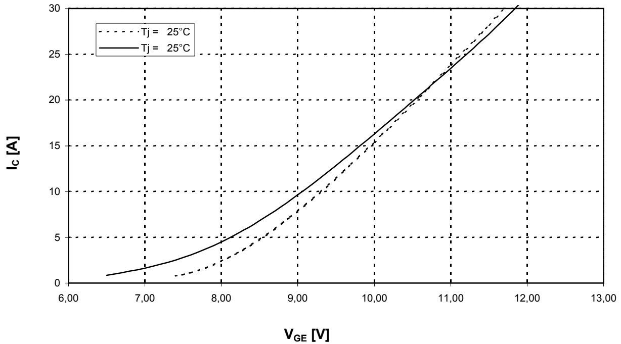
transfer characteristic inverter (typical)
