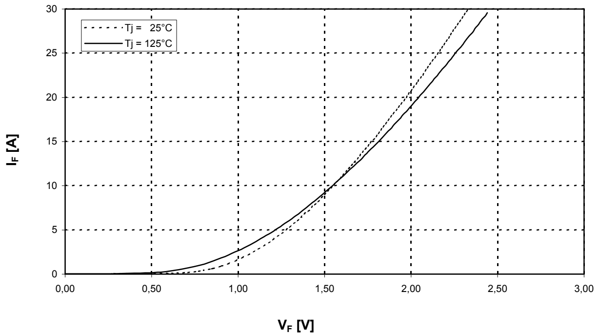
forward characteristic of FWD inverter (typical)
